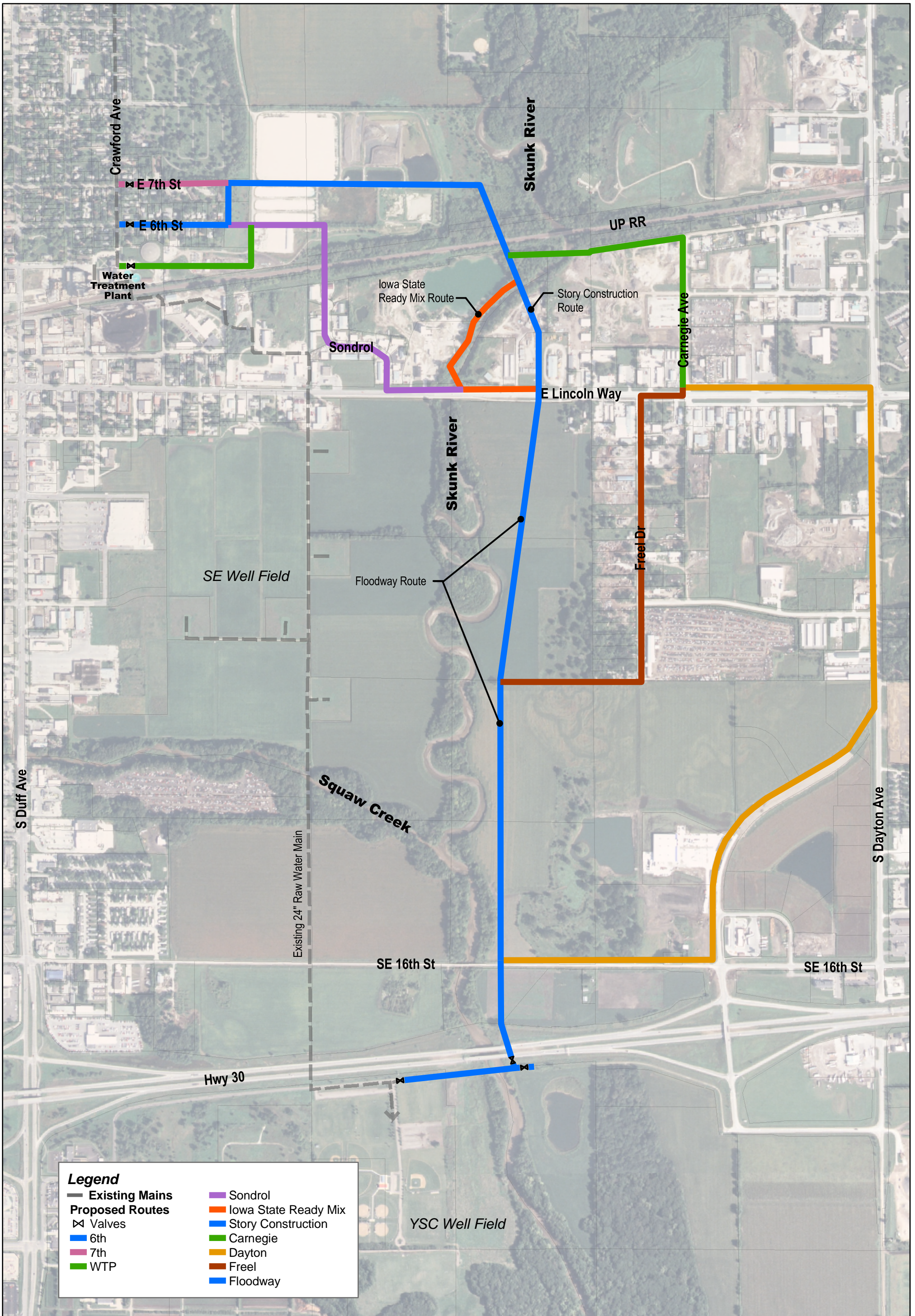
FIGURE 1: Alternate Routes Raw Well Water Transmission Pipeline Water & Pollution Control Department Ames, Iowa
